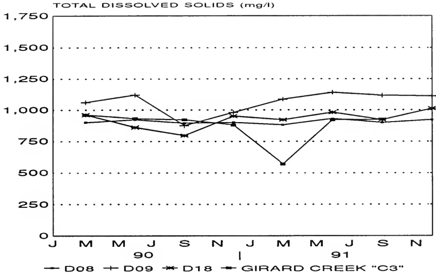
Figure 4.3 TDS for Selected Discharge Points, 1990 and 1991.
